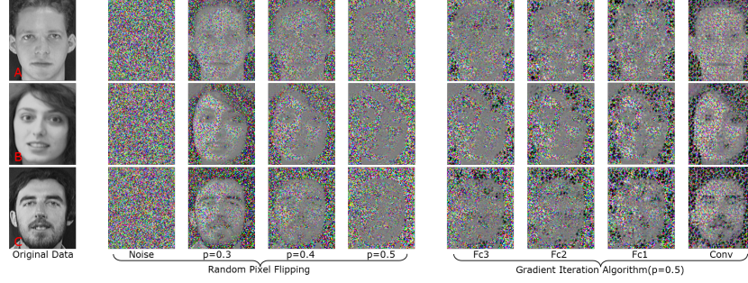
Fig. 3: Ablation. Examples for \tilde{X} that are generated with different p and F(\cdot)
