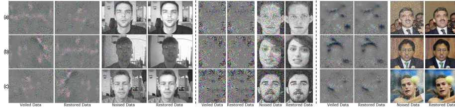
Fig. 5: Image Restoration Method (GPEN) on BioID, ORL and LFW
