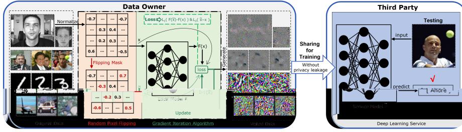
Fig. 1: The Veil Privacy framework and its application for visual privacy protection. (1) Veiled Data Generation . The data owner generates the veiled data from the original data via Veil Privacy and then shares them with the third party without visual privacy leakage. (2) Application . The third party trains the DNN model using the shared veiled data to provide deep learning services. Then the trained service model can effectively predict not only the veiled data but also the original data during the testing phase.
